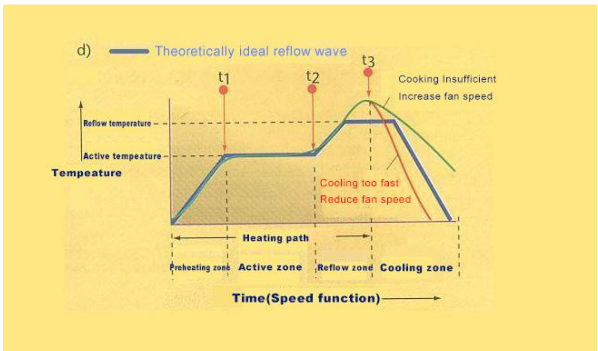
Figure 6: Cooling too much/little
