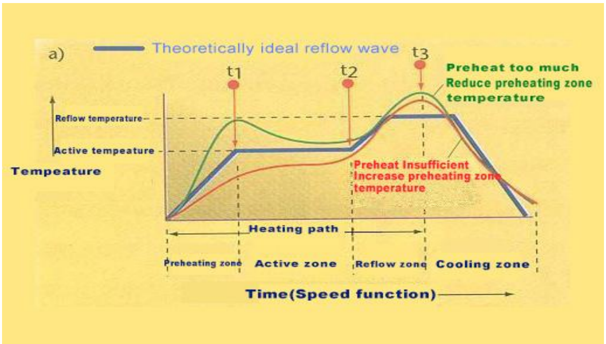
Figure 3: Preheat too much/little soldering profile
