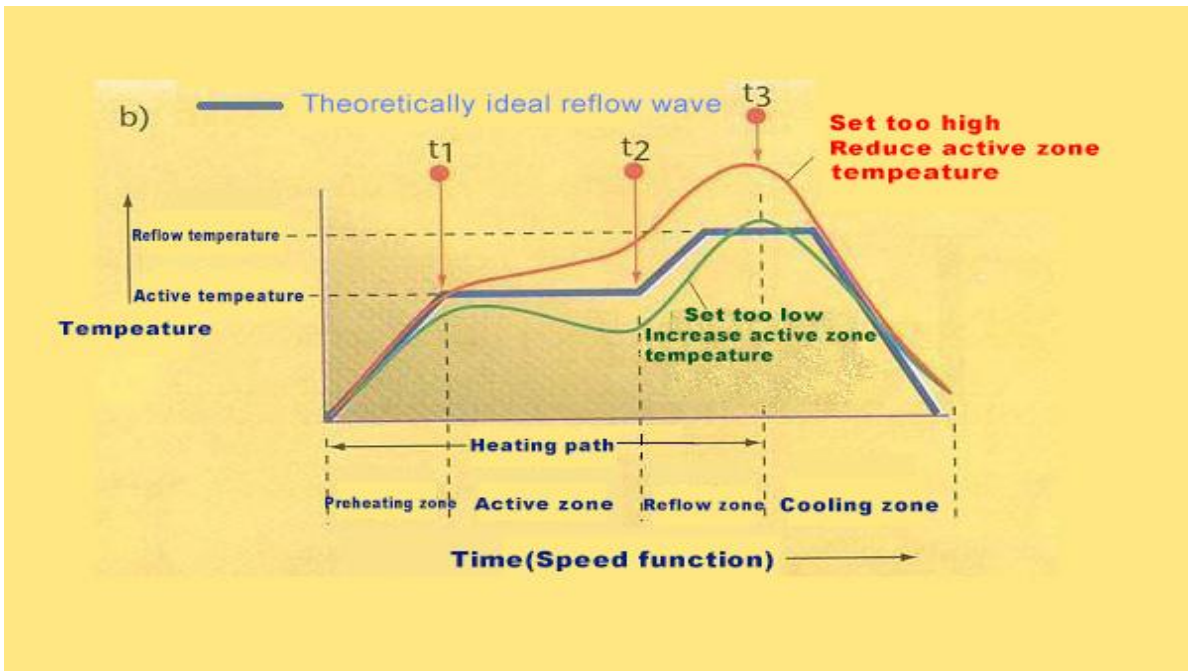
Figure 4: Set too high/low temperature of Active zone
