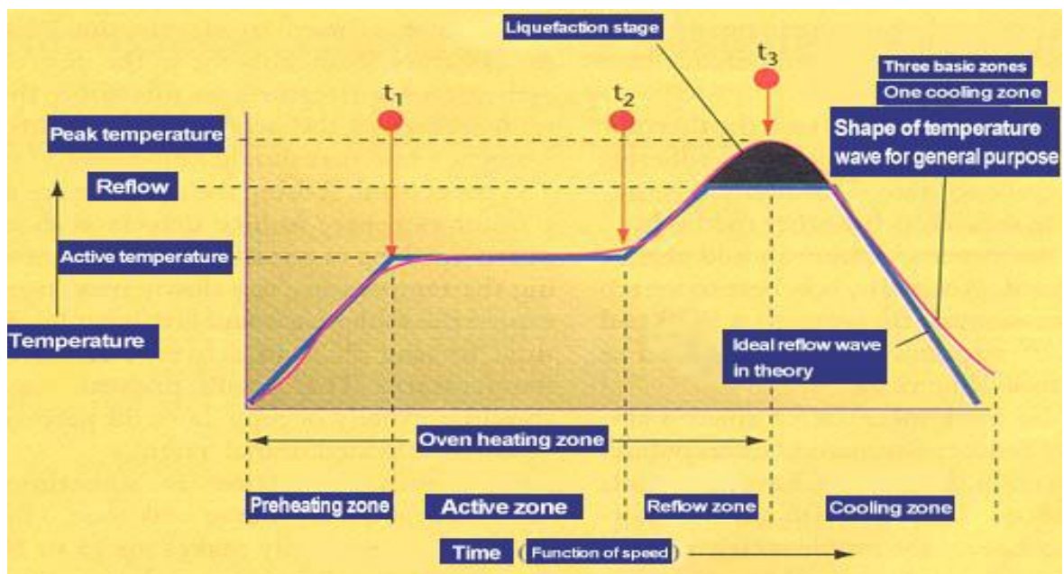
(Fig. 2. Theoretically, the ideal reflow curve consists of four zones, the first three zones are heating and the last zone is cooling.)
