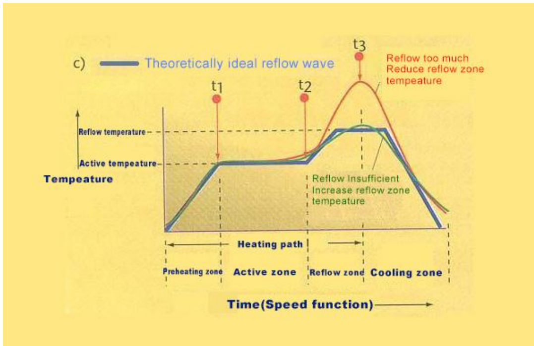
Figure 5: Soldering (Reflow Zone) too much/little
